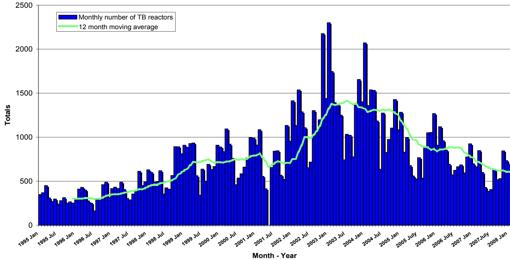
TB Reactors: January 1995 to January 2008
