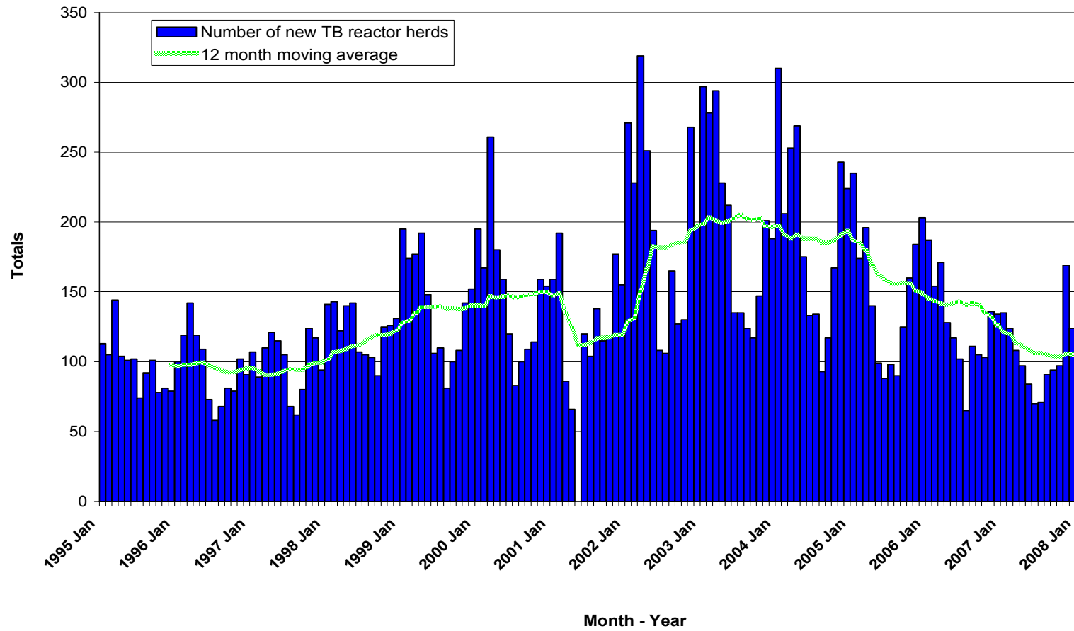
New TB Reactor Herds: January 1995 to January 2008
